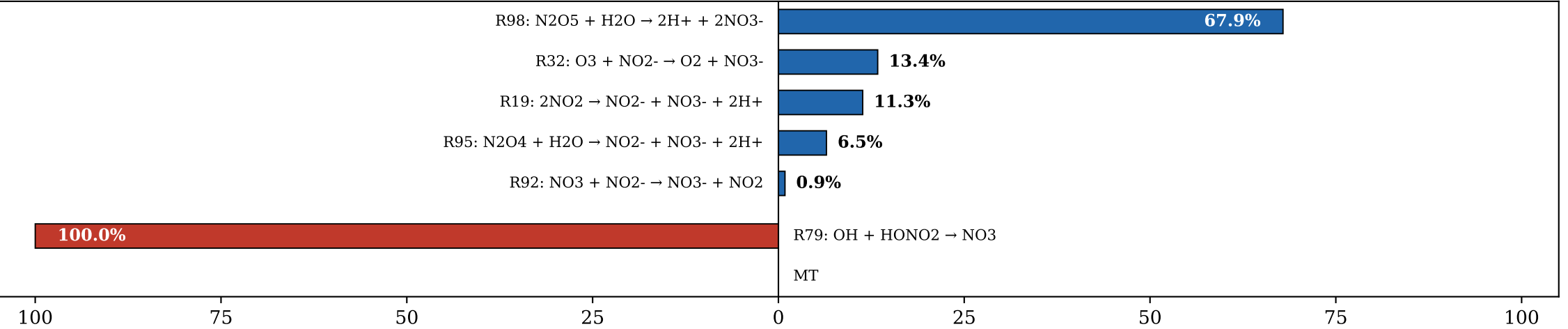
(b) O 3 (Σsrc = 4.60e-08 M/s)
