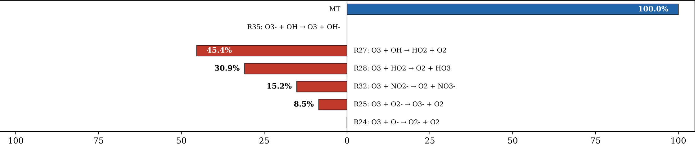
(c) NO 2 - (Σsrc = 8.48e-09 M/s)
